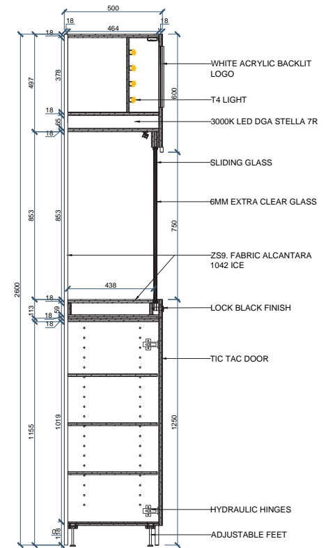
BACKWALL SIDE SECTION
