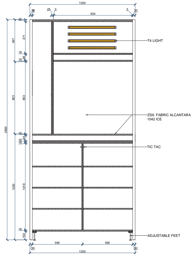
BACKWALL FRONT SECTION
