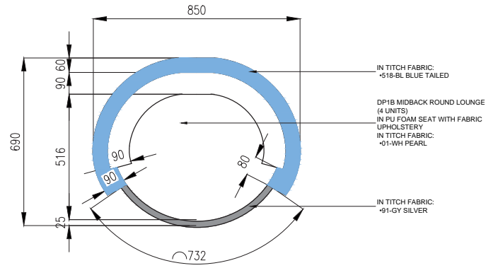
A TOP VIEW 00 SCALE 1 : 16
