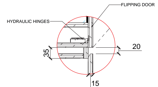
04 SECTION H DETAIL 03 SCALE 1:3
