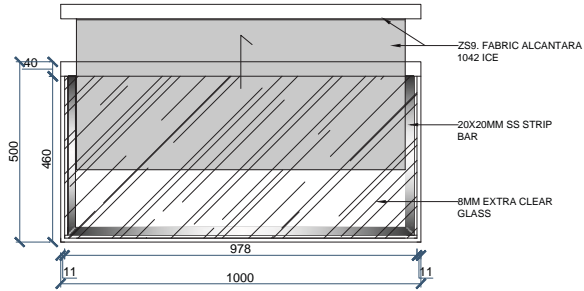
COUNTER TOP VIEW
