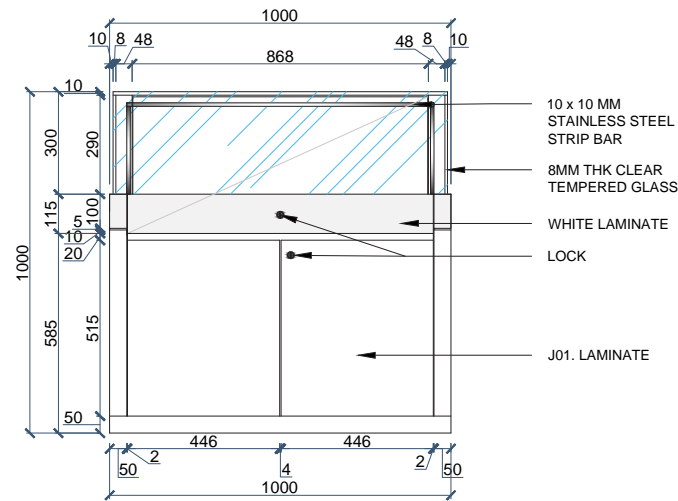
COUNTER REAR VIEW
