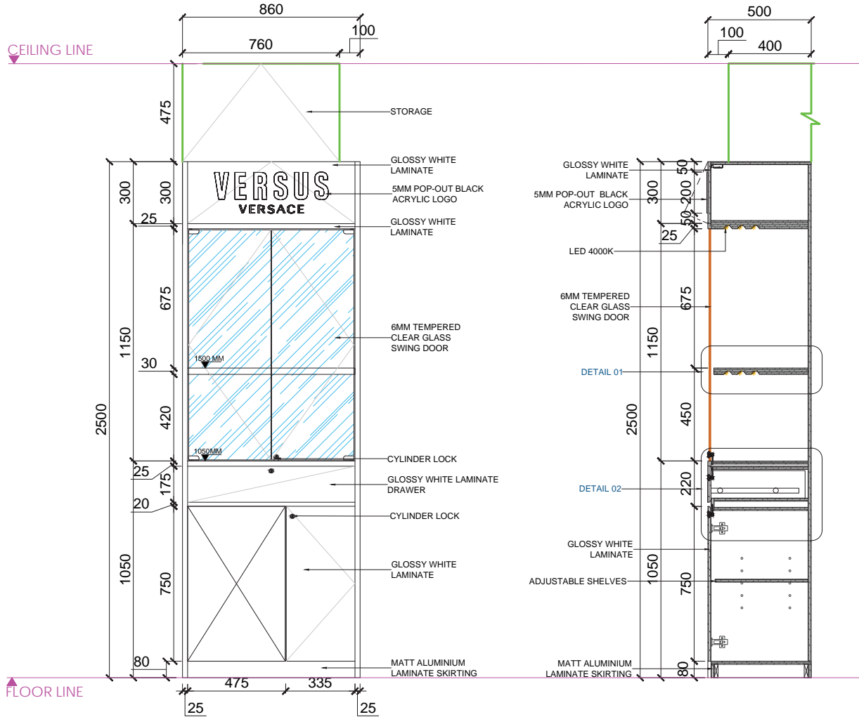
01 SECTION A-A FRONT VIEW
