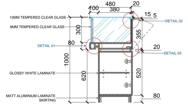
02 SECTION H SIDE VIEW
