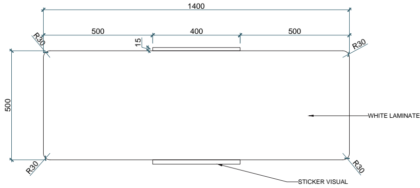
01 DISPLAY COUNTER TOP VIEW
