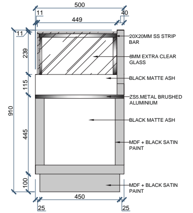
COUNTER SIDE VIEW
