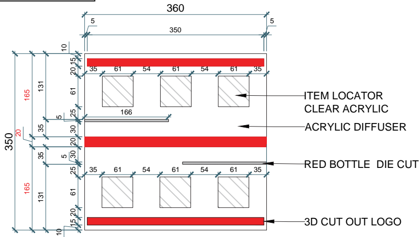
01 ACRYLIC TESTER DISPLAY TOP VIEW
