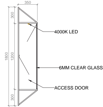
DETAIL 01 SIDE
