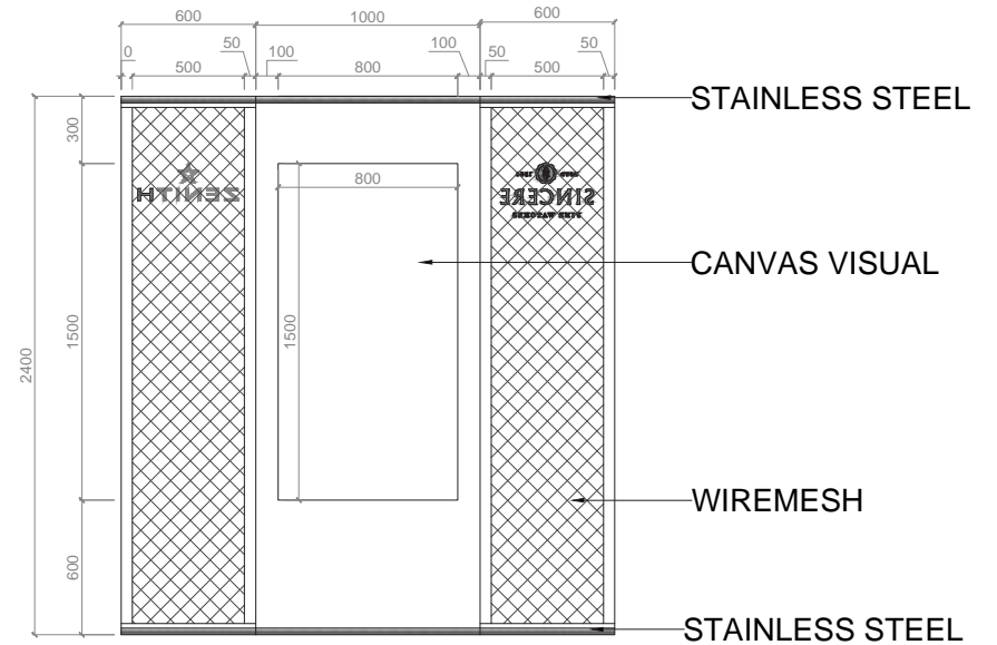
ELEVATION B DISPLAY BACKWALL
