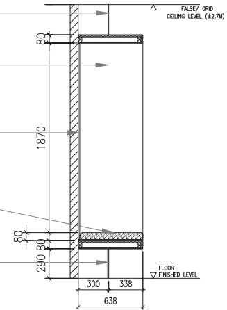
SEC SECTION J10 SCALE 1 : 40
