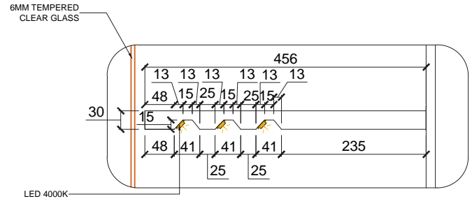
03 SECTION A-A DETAIL 1 SCALE 1:3
