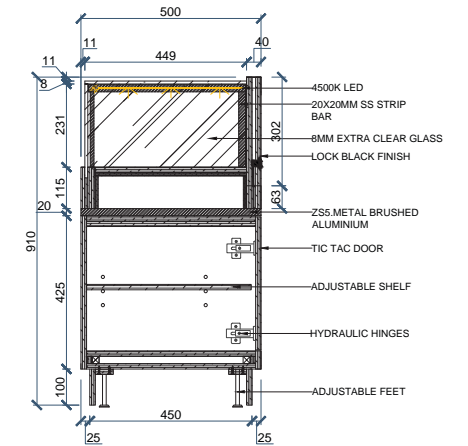
COUNTER SIDE SECTION
