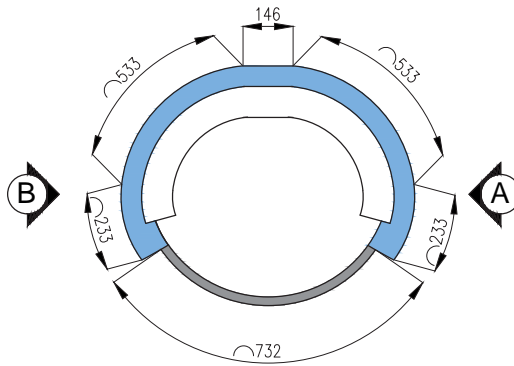
B TOP VIEW 00 SCALE 1 : 16
