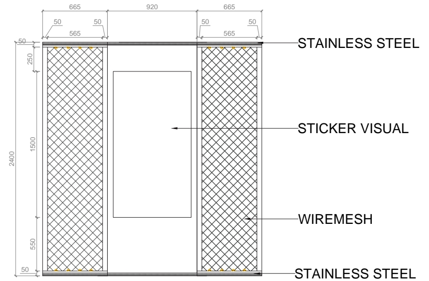
ELEVATION B DISPLAY BACKWALL
