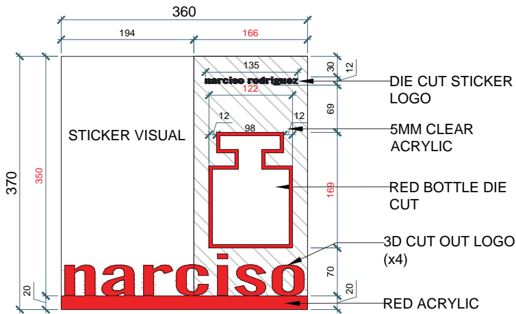
01 ACRYLIC TESTER DISPLAY TOP VIEW
