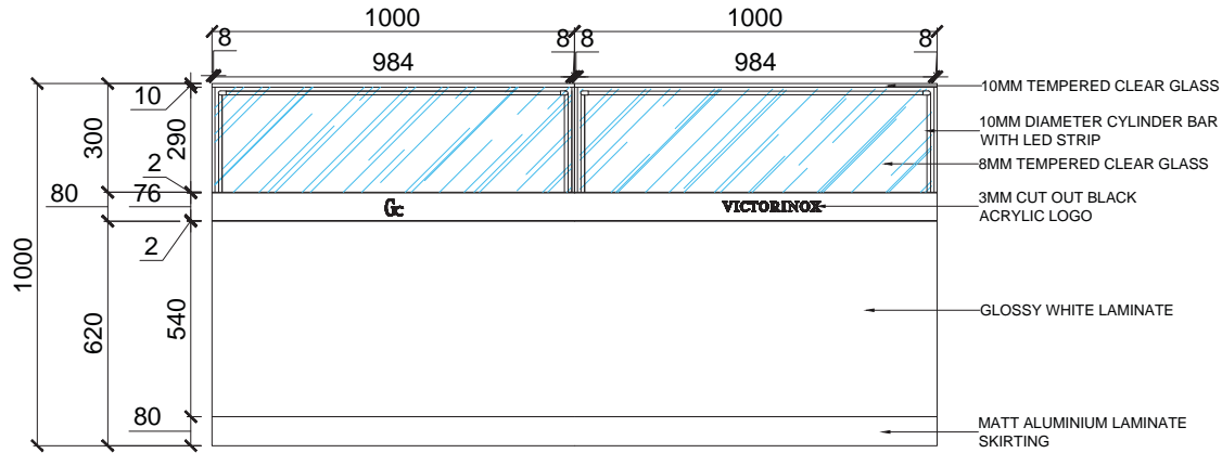
01 SECTION H FRONT VIEW
