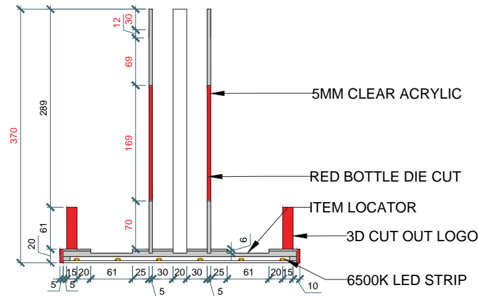
04 ACRYLIC TESTER DISPLAY SIDE SECTION
