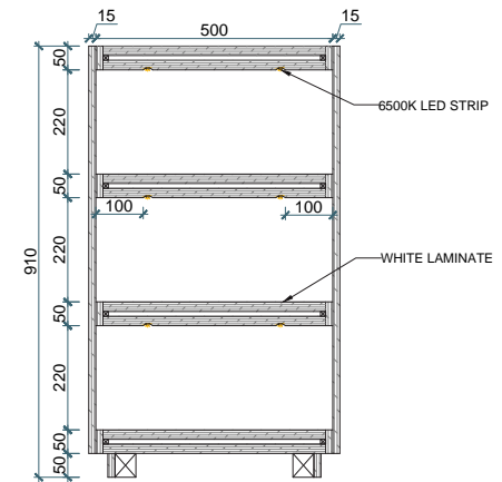
04 DISPLAY COUNTER SIDE SECTION
