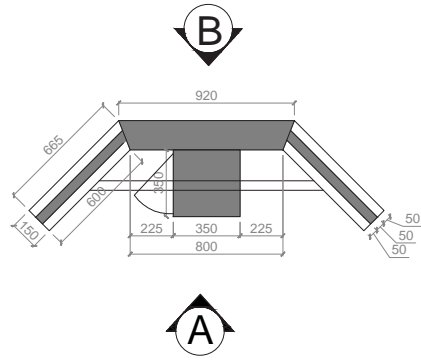
TOP VIEW DISPLAY BACKWALL
