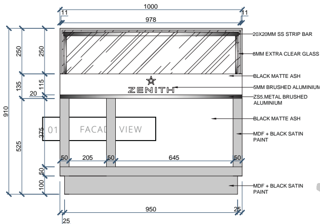
COUNTER FRONT VIEW
