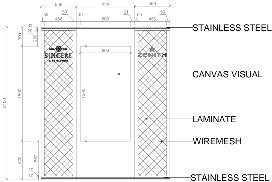
ELEVATION A DISPLAY BACKWALL
