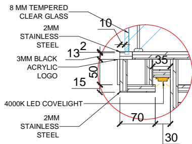
03 SECTION H DETAIL 01 SCALE 1:3
