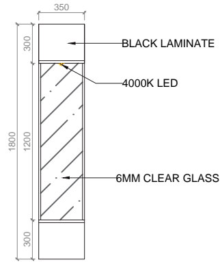
DETAIL 01 FRONT
