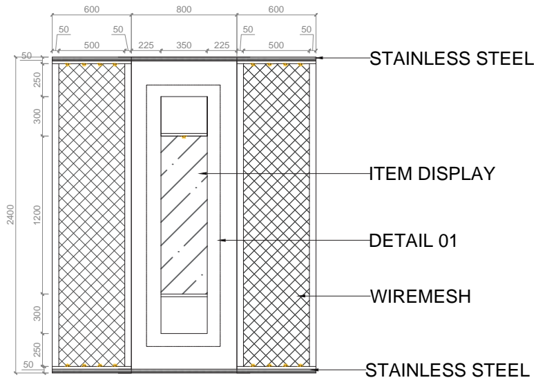
ELEVATION A DISPLAY BACKWALL
