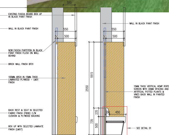
SEC SIDE VIEW J08 SCALE 1:30
