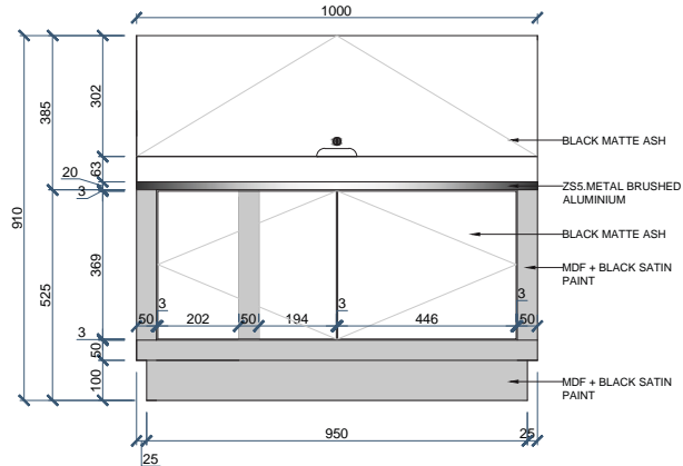
COUNTER REAR VIEW
