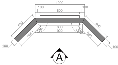
TOP VIEW VISUAL BACKWALL
