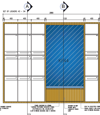
SEC 114 FRONT ELEVATION SCALE 1 : 20
