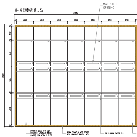
SEC 114 FRONT ELEVATION SCALE 1 : 20
